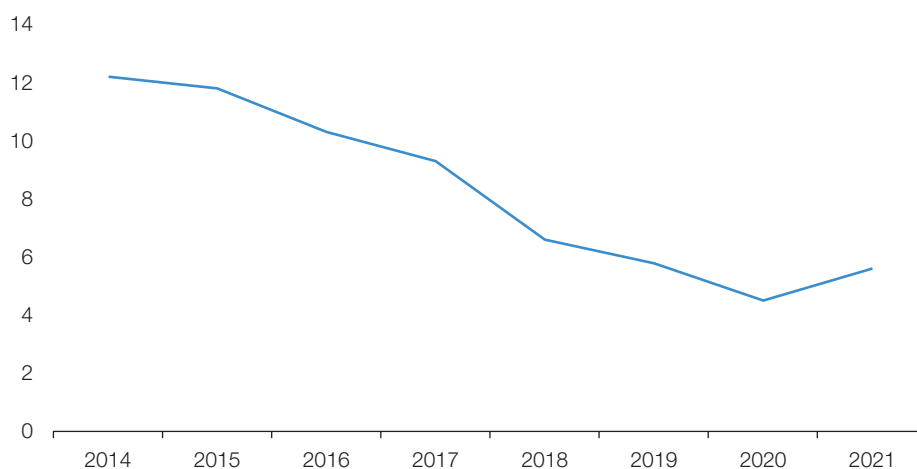
CRE Overall Curtailment Rate (%) 中國再生能源總體限電率(%)
